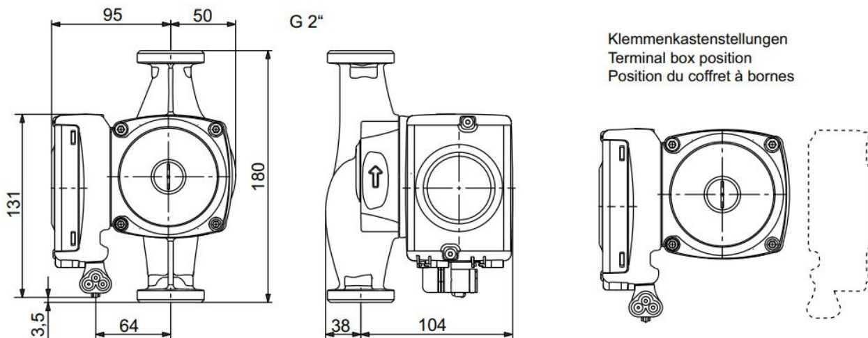
Dimension drawing
