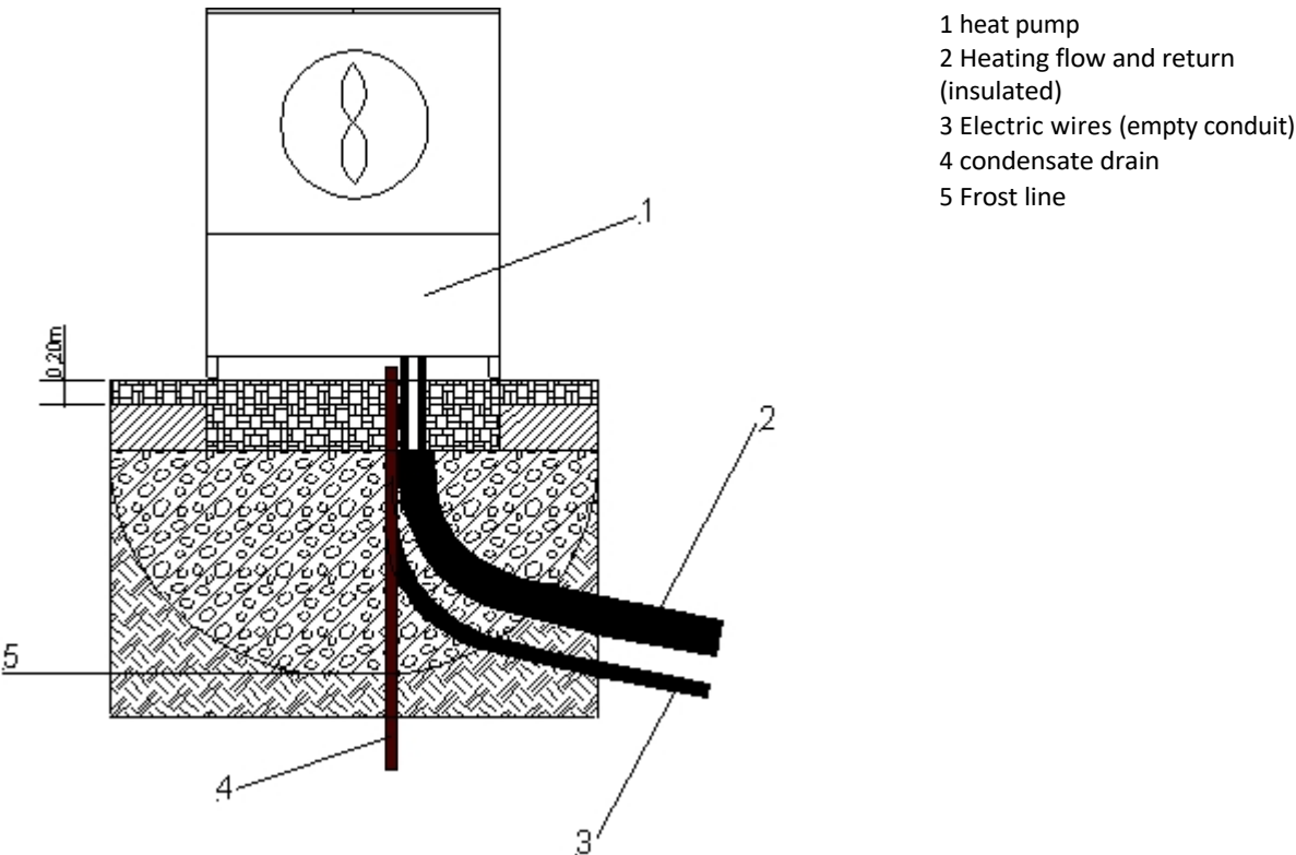
8 Illustration: Foundation plan for heat pump with condensate drain
