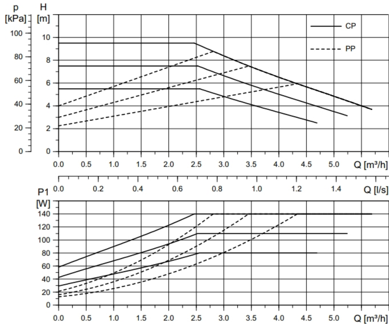
Diagrams/characteristic curve
