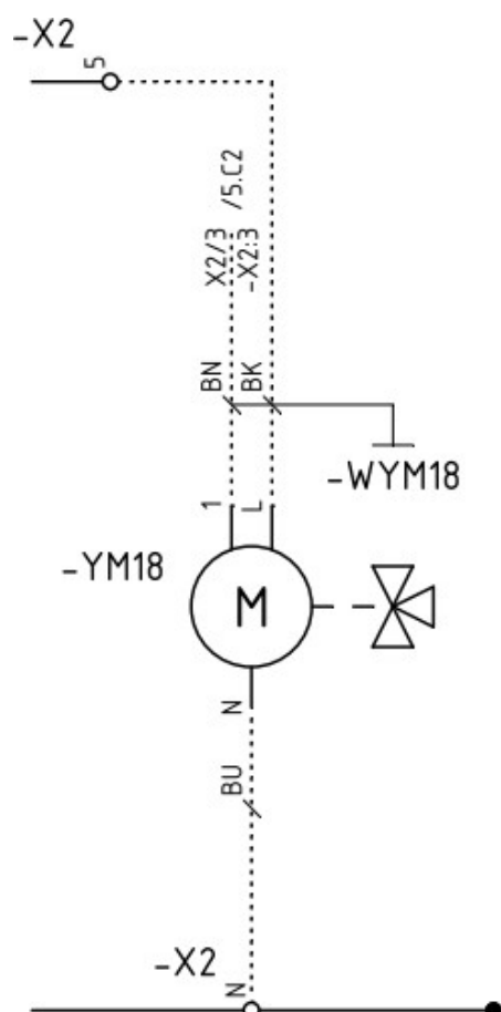
42 Connection diagram 2-point control
