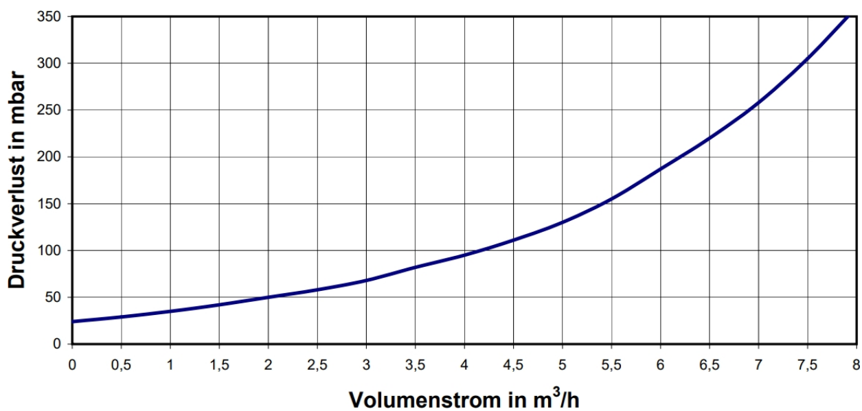
Volume flow pressure drop diagram DDV 50
